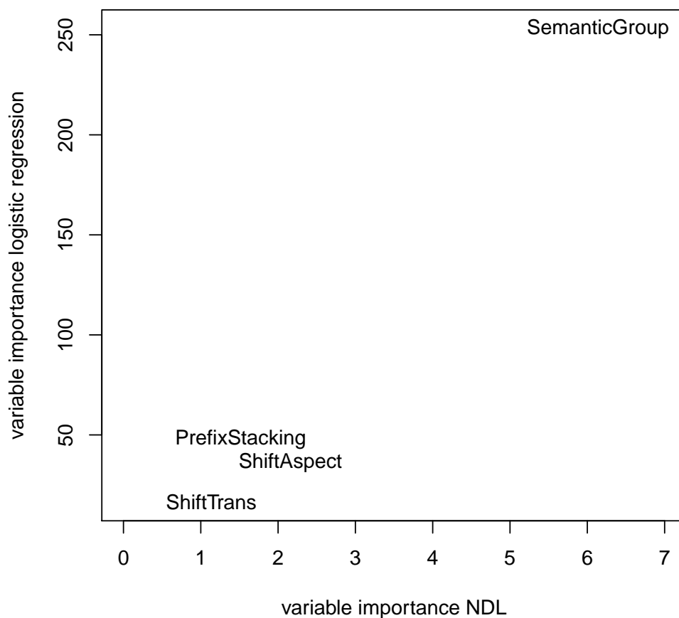
Figure 4: Variable importance according to the logistic regression model and according to naive discriminative learning for the nepe- vs. npe- dataset.
