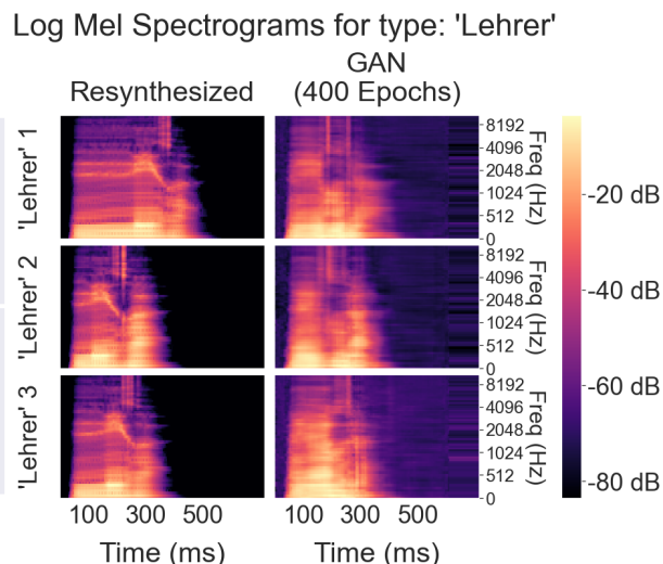
Figure 4 – Log-mel spectrograms generated by the Mel-GAN for the word “Lehre” in comparison to segment-based syntheses.
