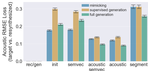
Figure 1 – Mean RMSE loss between final produced and target acoustic for the semvec, acoustic semvec, and acoustic objective. Init refers to the initial cp-trajectory.
